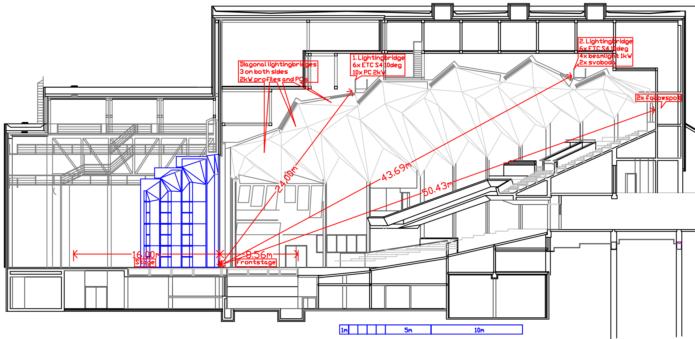
TAMPERE-TALO - Main auditorium - cross-section Location of frontlights
